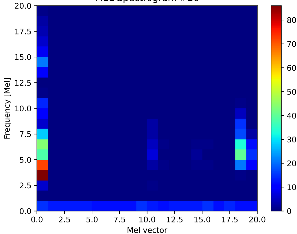
MEL Spectrogram #20
